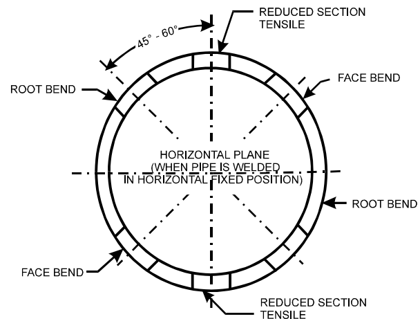
Figure 5.22 — Location of Test Specimens for Job Size Pipe or Tubing 1/16 in. through 3/8 in. Wall Thickness (see 5.17.4.3)
