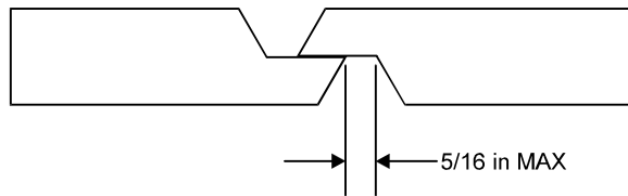
(B) ROOT OPENING ON SLIP-FIT JOINTS
