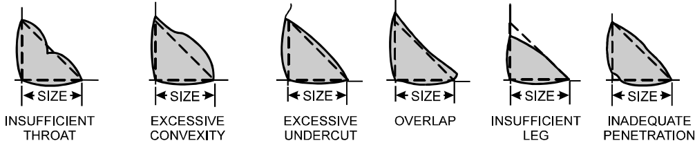
(C) UNACCEPTABLE WELD PROFILES
