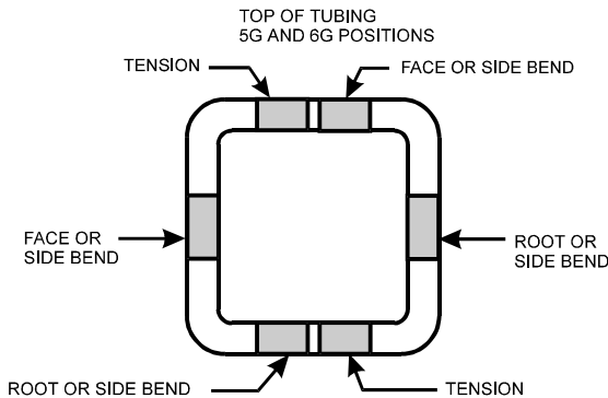
Figure 5.21 — Location of Test Specimens for Square and Rectangular Tubing (see 5.17.4.3)
