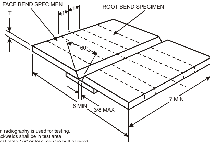
Figure 5.26 — Test Plate for Limited Thickness — All Positions — Performance Qualification (see 5.21.2)
