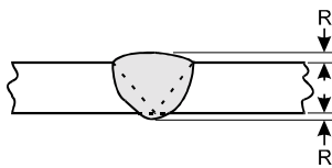
(E) ACCEPTABLE PROFILE: GROOVE WELD IN BUTT JOINT WELDED FROM ONE SIDE
