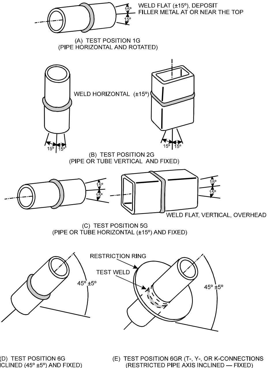
Figure 5.4 — Position of Test Plate for Groove Welds (see 5.6.1.2)
