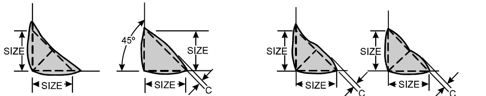
(A) DESIRABLE WELD PROFILES
