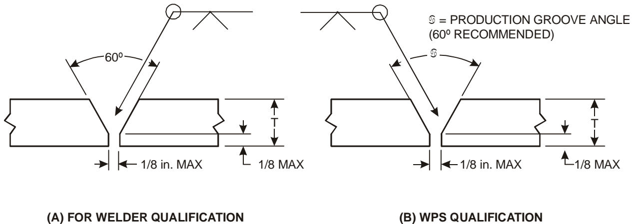
Figure 4.7 — Tubular Butt Joint — Welder or WPS Qualification — without Backing (see Table 4.5)
