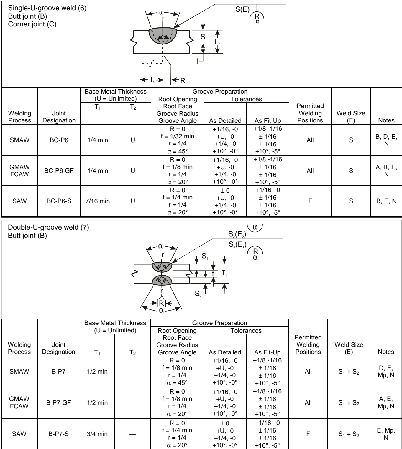
Figure E.1 (Sheet 4) — Prequalified Partial Joint Preparation (PJP) Groove Welded Joint Details (see 3.8) Top — Single U-groove weld, butt or corner joint Bottom — Double U-groove weld, butt joint
