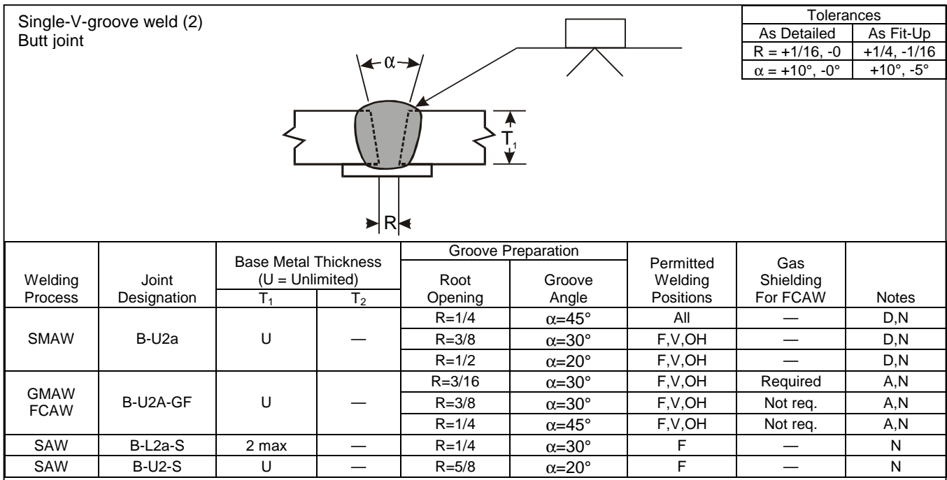
Figure E.2 (Sheet 2) — Prequalified Complete Joint Preparation (CJP) Groove Welded Joint Details (see 3.9) Top — Square-groove weld, T- or corner joint Bottom — Single-V-groove weld, butt joint
