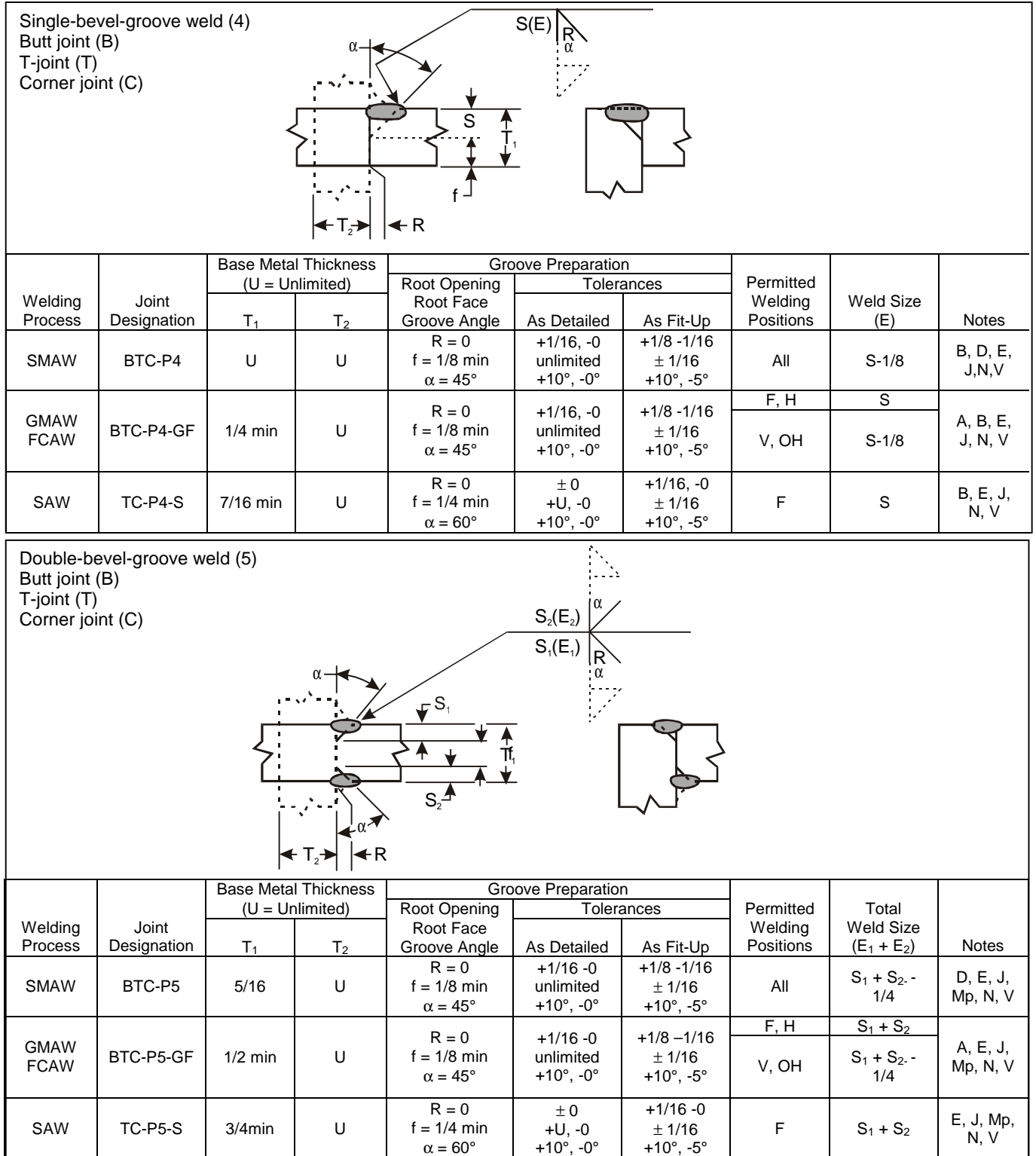
Figure E.1 (Sheet 3) — Prequalified Partial Joint Preparation (PJP) Groove Welded Joint Details (see 3.8) Top — Single-bevel-groove weld, butt, or T-, or corner joint Bottom — Double bevel-groove weld, butt, or T-, or corner joint
