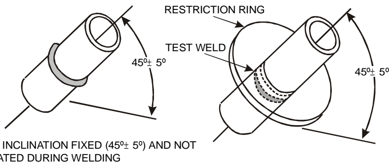
(E) TEST POSITION 6GR (T-, Y-, OR K-CONNECTION)
